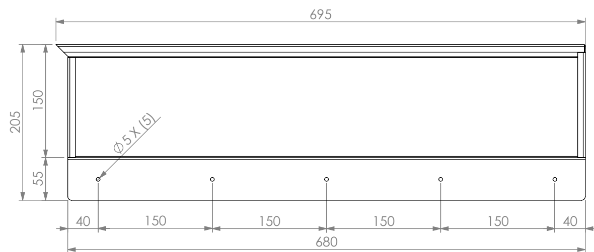
FRONT ELEVATION
